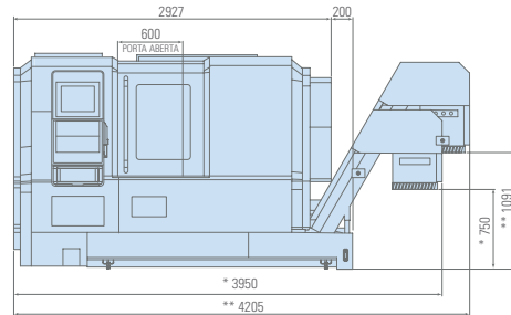
VISTA FRONTAL
